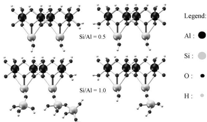
Fig. 9. Structure of nano-ball allophane around the defect sites. Redrawn from Ref. [12].
