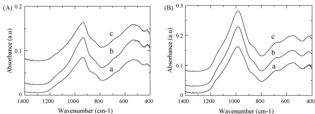
Fig. 5. FTIR spectra of allophane precipitates. (A) Allophane with initial Si/Al ratio of 0.67 reacted with arsenate. (B) Allophane with initial Si/Al ratio of 1.0 reacted with B. Note: (a) Allophane without sorbed anions; (b) after adsorption and (c) after co-precipitation.
