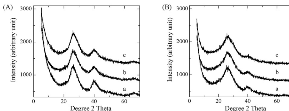
Fig. 4. XRD profiles of boric acid reacted allophanes. (A) B sorption with initial Si/Al ratio = 0.67. (B) B sorption with initial Si/Al ratio = 1.0. Note: (a) Without sorbed anions, (b) after adsorption, and (c) after co-precipitation.
