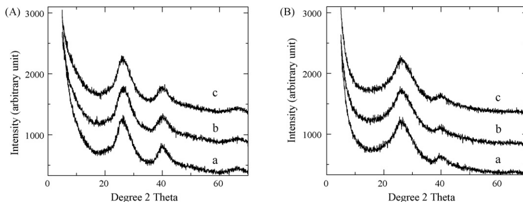
Fig. 3. XRD profiles of arsenate reacted allophanes. (A) As sorption with initial Si/Al ratio = 0.67. (B) As sorption with initial Si/Al ratio = 1.0. Note: (a) Without sorbed anions, (b) after adsorption, and (c) after co-precipitation.
