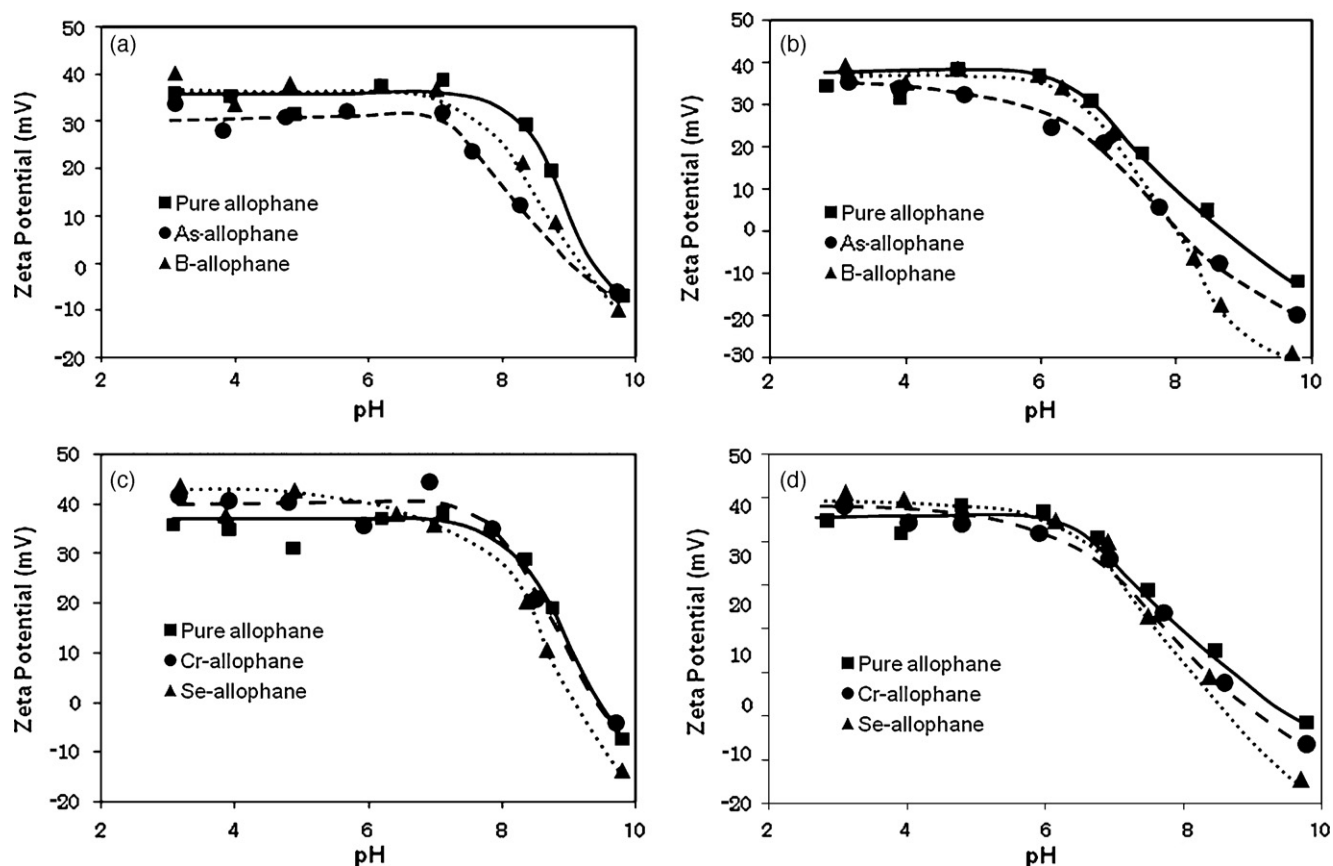
Fig. 8. Surface charge characteristics of allophane samples after adsorption. (A and C) Allophane with initial Si/Al ratio = 0.67. (B and D) Allophane with initial Si/Al ratio = 1.0.
