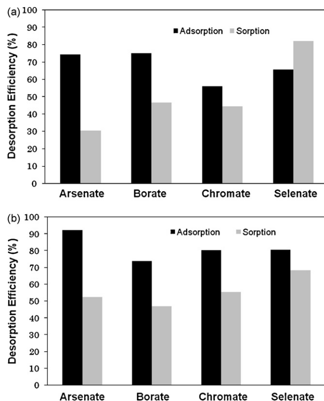
Fig. 7. Desorption efficiency of oxyanions after phosphate extraction. (A) Allophane with lower final Si/Al ratio. (B) Allophane with higher final Si/Al ratio.
