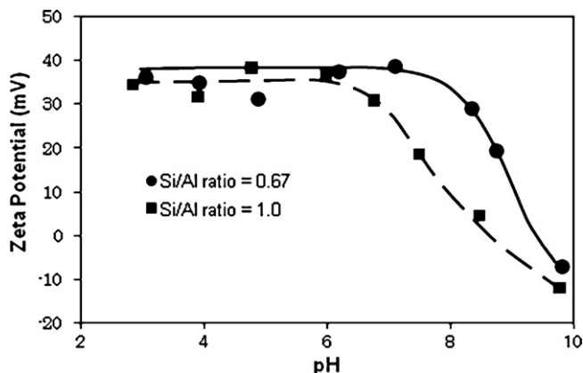
Fig. 6. Surface charge characteristics of allophane without sorbed anions.
