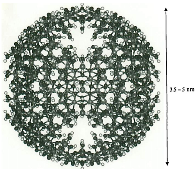
Fig. 1. Structural model of allophane. Reproduced after Ref. [12] with permission from The Clay Science Society of Japan.
